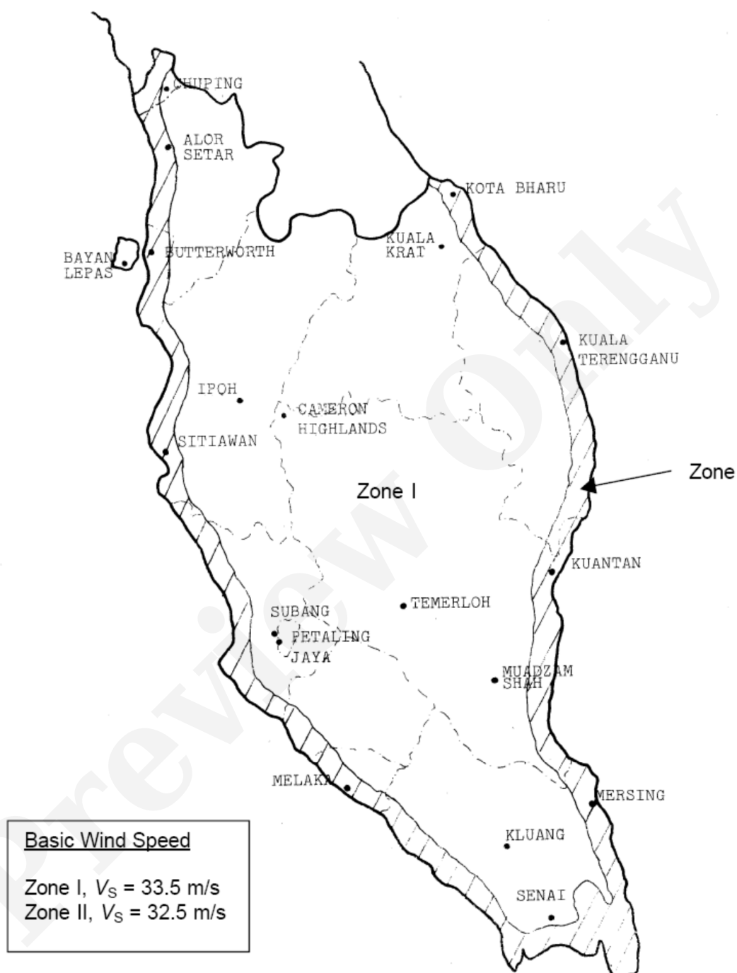
Figure 3.1 Basic Wind Speed for Peninsular Malaysia (Simplified Procedures)
